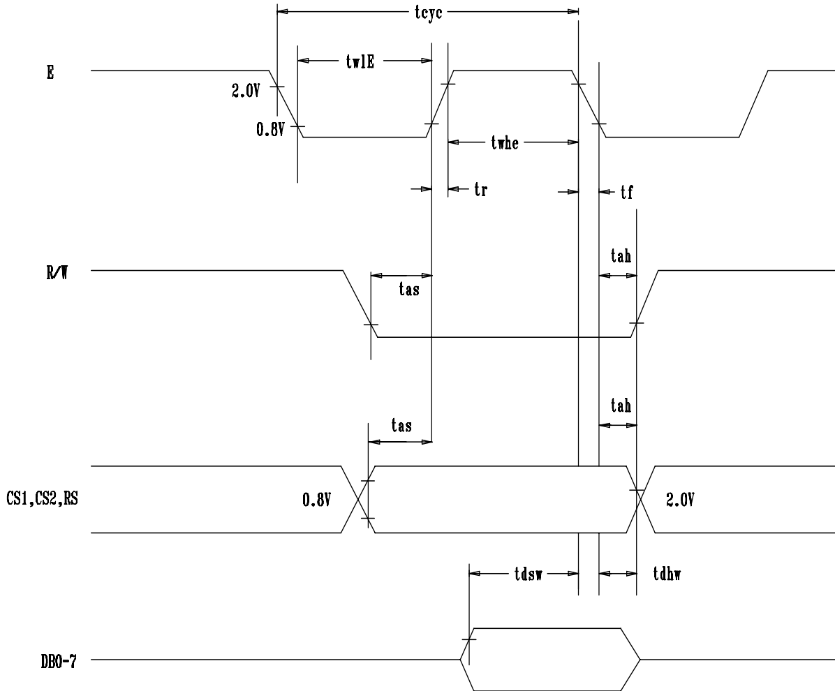
MPU Write Timing
